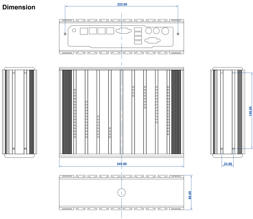
2 PCI Slot Chassis
